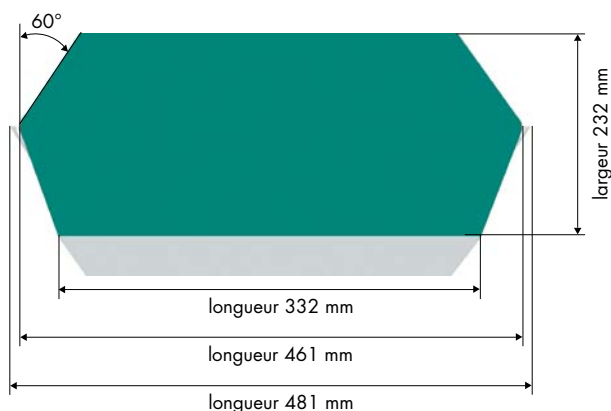
Figure 2 : Dimensions.
